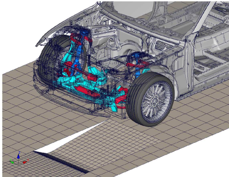
Figure 3: A possible MBS–FEA coupling setup.
